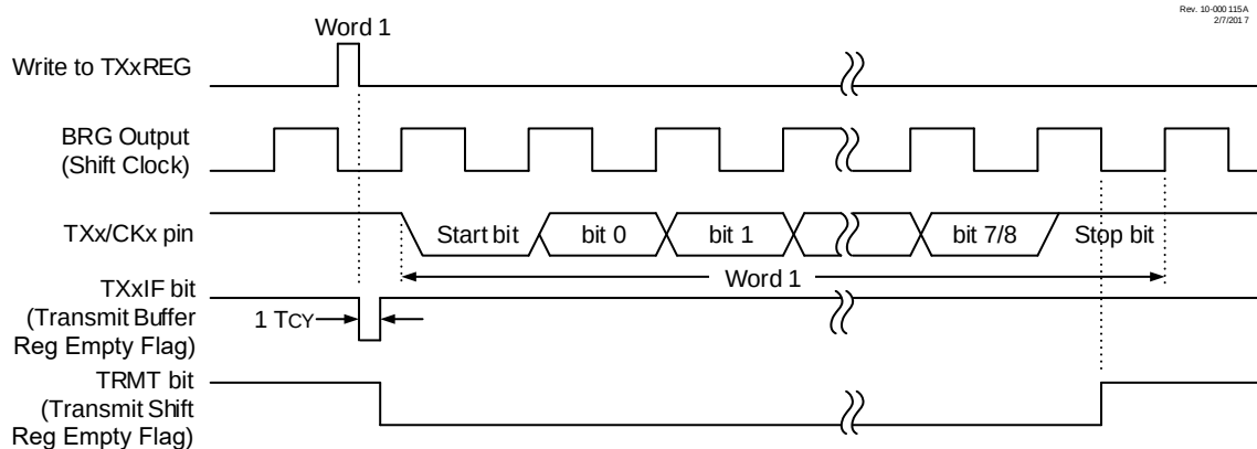
Figure 24-10. Synchronous Transmission
