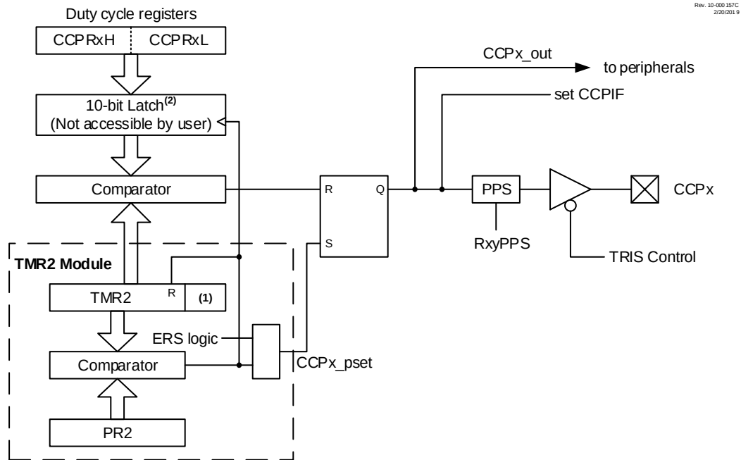
Figure 22-4. Simplified PWM Block Diagram
