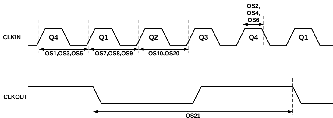
Figure 32-4. Clock Timing
