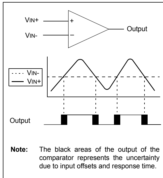
FIGURE 16-1: SINGLE COMPARATOR
