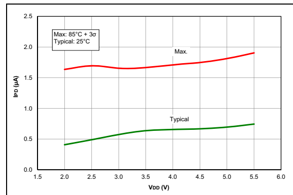
FIGURE 35-36: I_{PD} , Watchdog Timer (WDT), PIC16F1713/6 Only.
