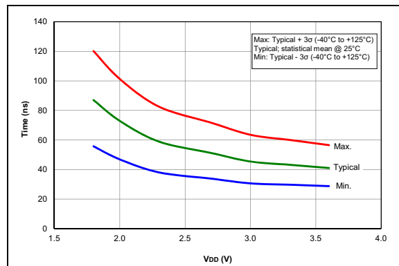
FIGURE 35-106: Comparator Response Time Over Voltage, NP Mode ( CxSP = 1 ), Typical Measured Values, PIC16F1713/6 Only.
