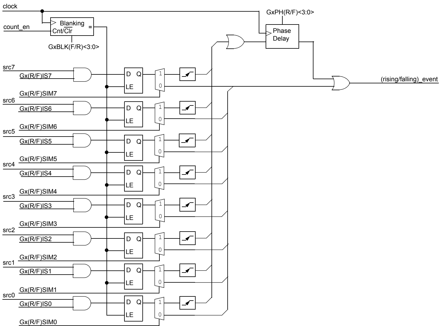
FIGURE 18-7: COG (RISING/FALLING) INPUT BLOCK
