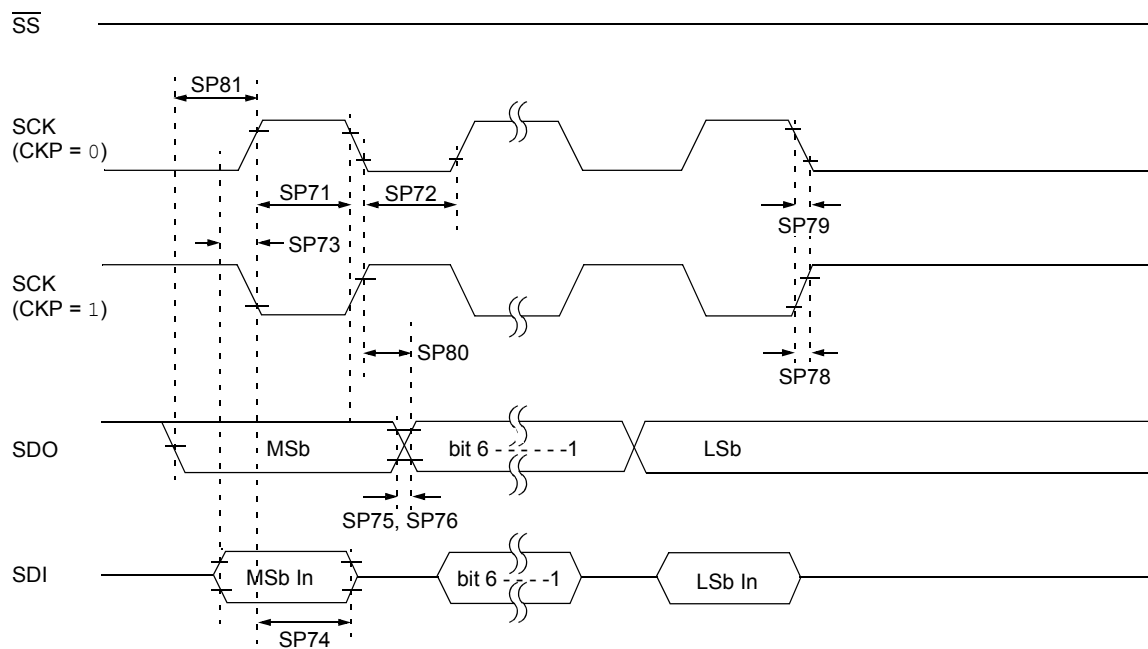
FIGURE 34-18: SPI MASTER MODE TIMING (CKE = 1, SMP = 1)
