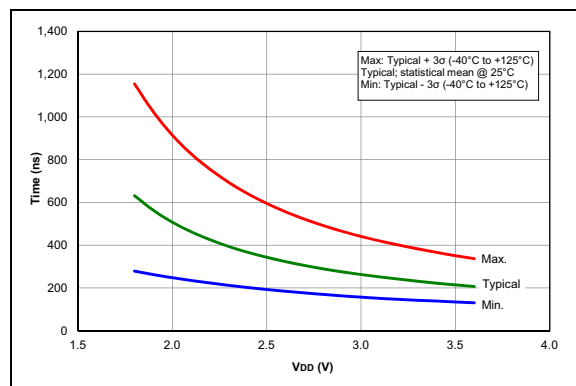
FIGURE 35-108: Comparator Output Filter Delay Time Over Temp., NP Mode ( CxSP = 1 ), Typical Measured Values, PIC16F1713/6 Only.
