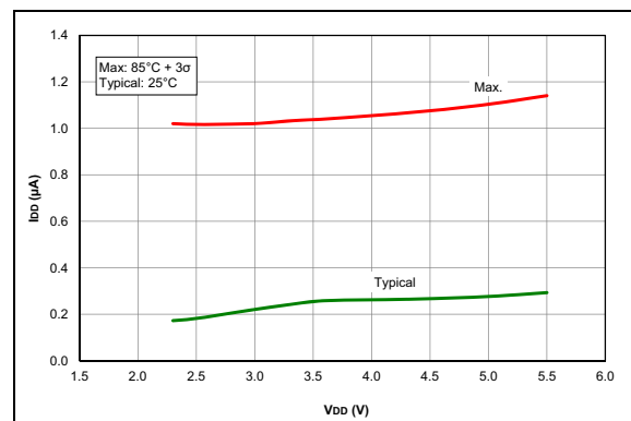
FIGURE 35-48: I_{PD} , ADC Non-Converting, PIC16F1713/6 Only.
