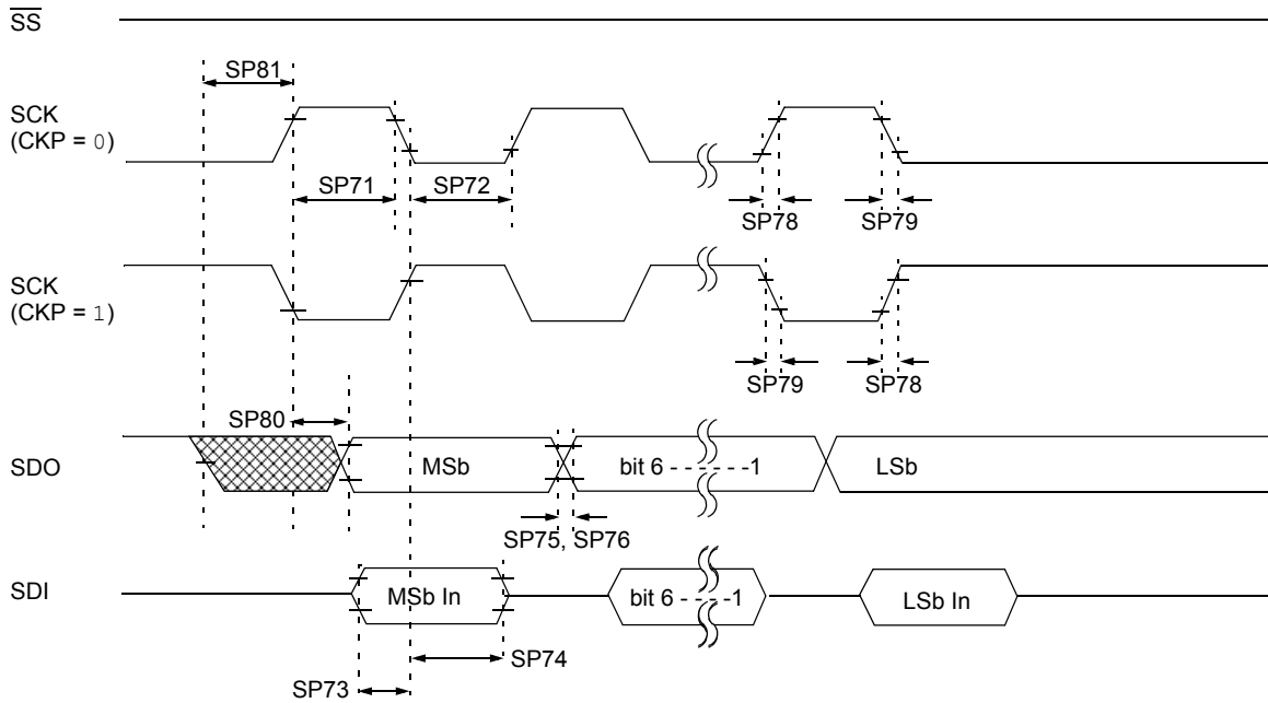
FIGURE 34-17: SPI MASTER MODE TIMING (CKE = 0, SMP = 0)
