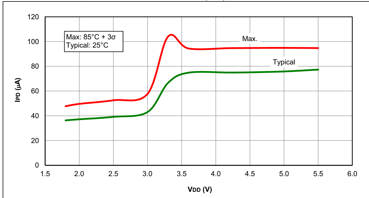
FIGURE 31-34: I_{PD} , FIXED VOLTAGE REFERENCE (FVR), PIC16F1933 ONLY
