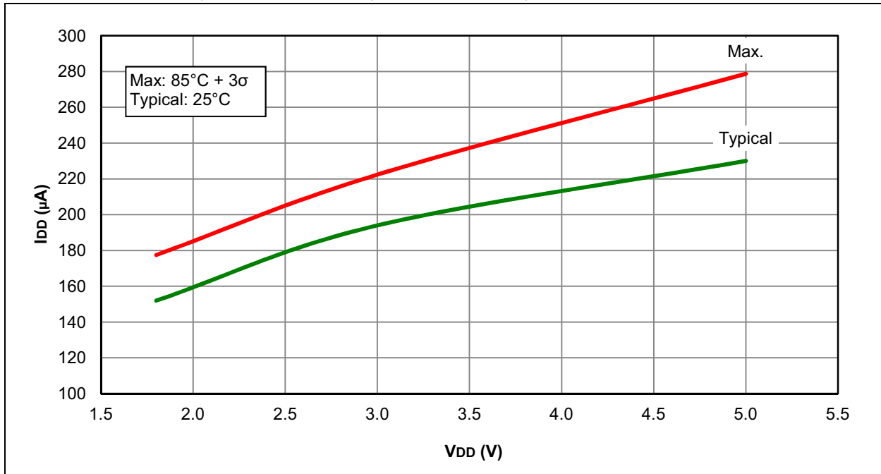
FIGURE 31-20: I_{DD} , MFINTOSC MODE, FOSC = 500 kHz, PIC16F1933 ONLY
