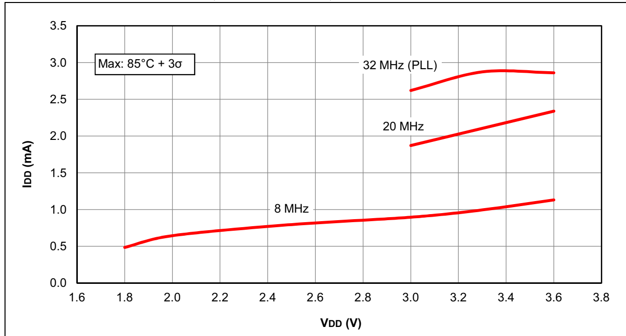
FIGURE 31-26: I DD MAXIMUM, HS OSCILLATOR, PIC16LF1933 ONLY
