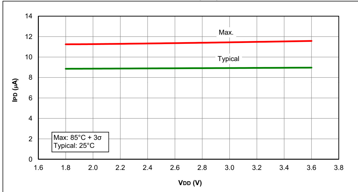
FIGURE 31-33: I_{PD} , FIXED VOLTAGE REFERENCE (FVR), PIC16LF1933 ONLY
