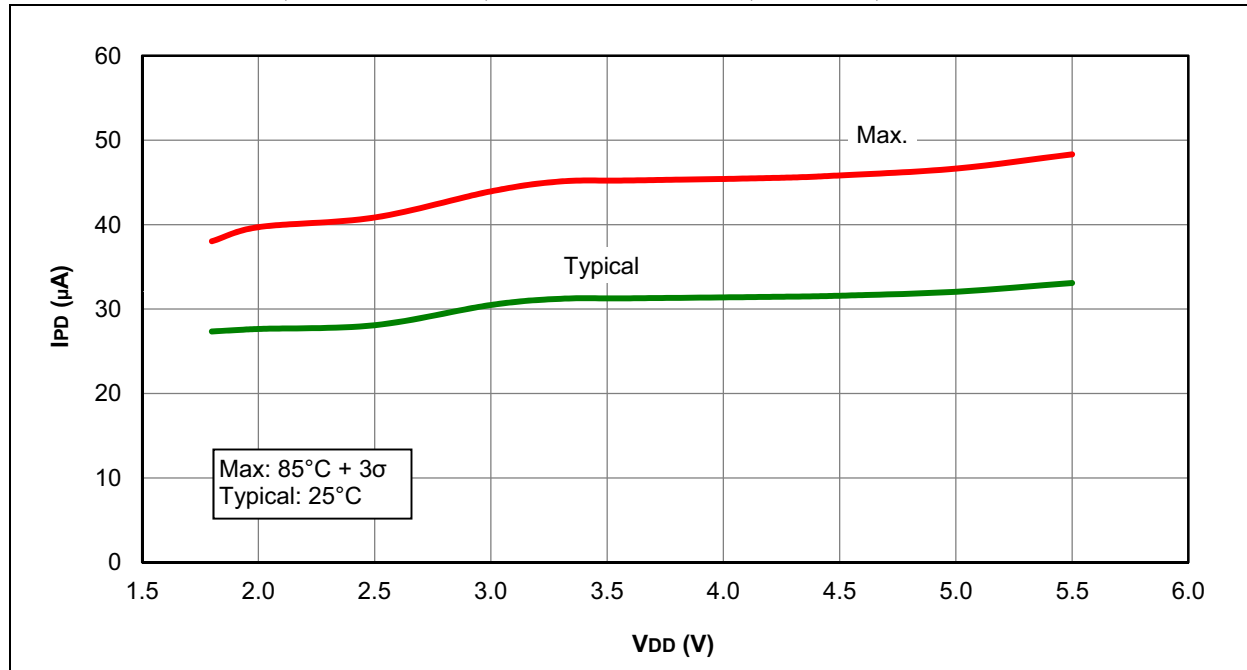
FIGURE 31-46: I_{PD} , COMPARATOR, LOW-POWER MODE, C_{xSP} = 0 , PIC16F1933 ONLY
