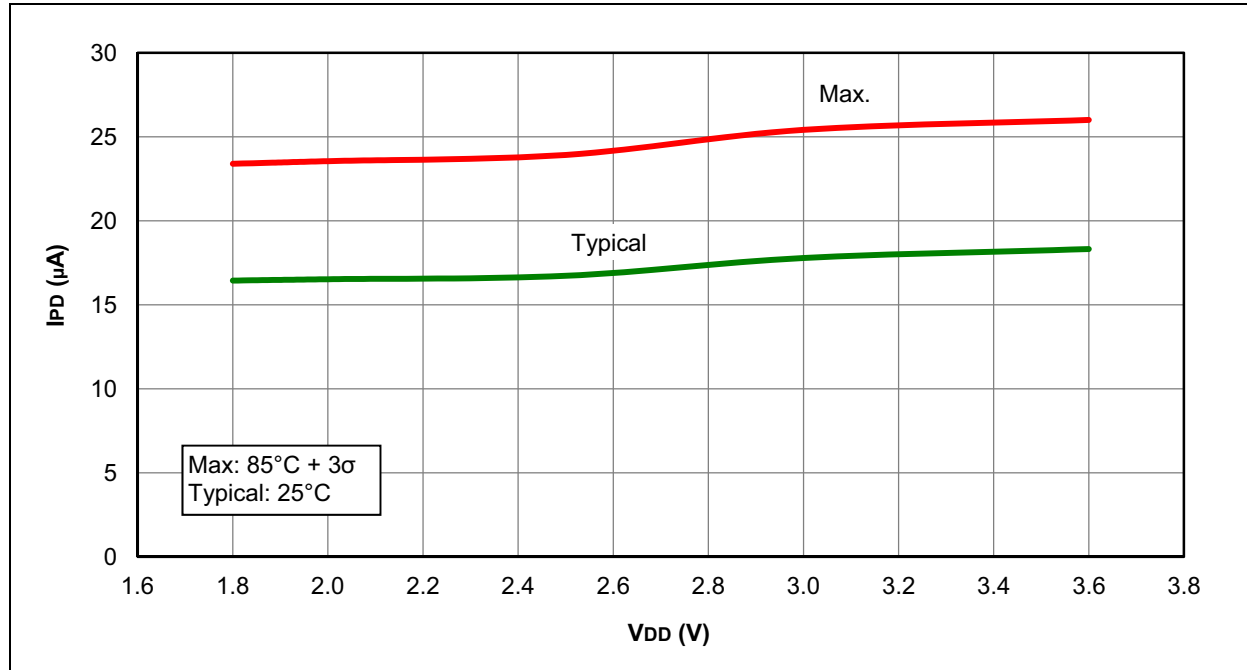
FIGURE 31-45: I_{PD} , COMPARATOR, LOW-POWER MODE, C_{xSP} = 0 , PIC16LF1933 ONLY
