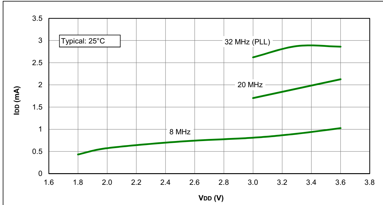
FIGURE 31-25: I DD TYPICAL, HS OSCILLATOR, PIC16LF1933 ONLY
