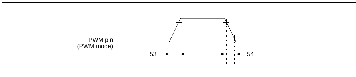
FIGURE 20-12: PWM TIMINGS
