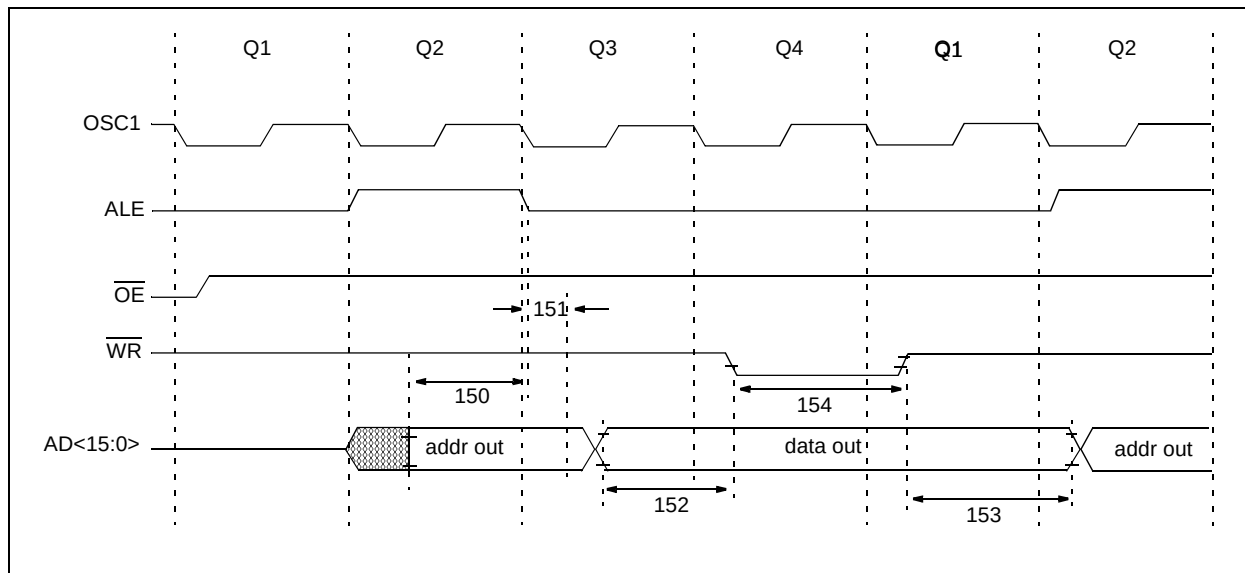
FIGURE 20-24: MEMORY INTERFACE WRITE TIMING
