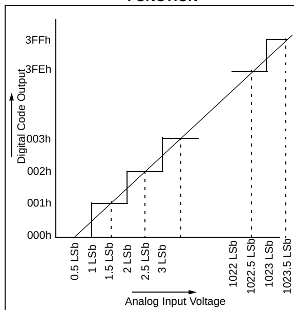
FIGURE 16-7: A/D TRANSFER FUNCTION
