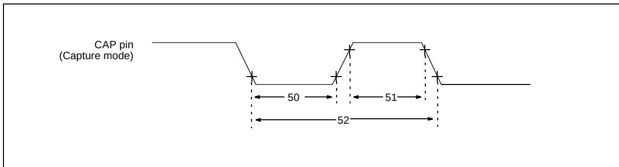
FIGURE 20-11: CAPTURE TIMINGS
