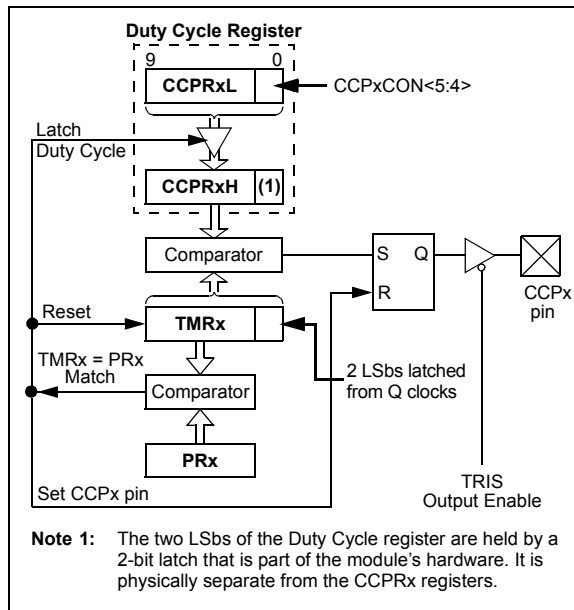
FIGURE 17-4: SIMPLIFIED PWM BLOCK DIAGRAM
