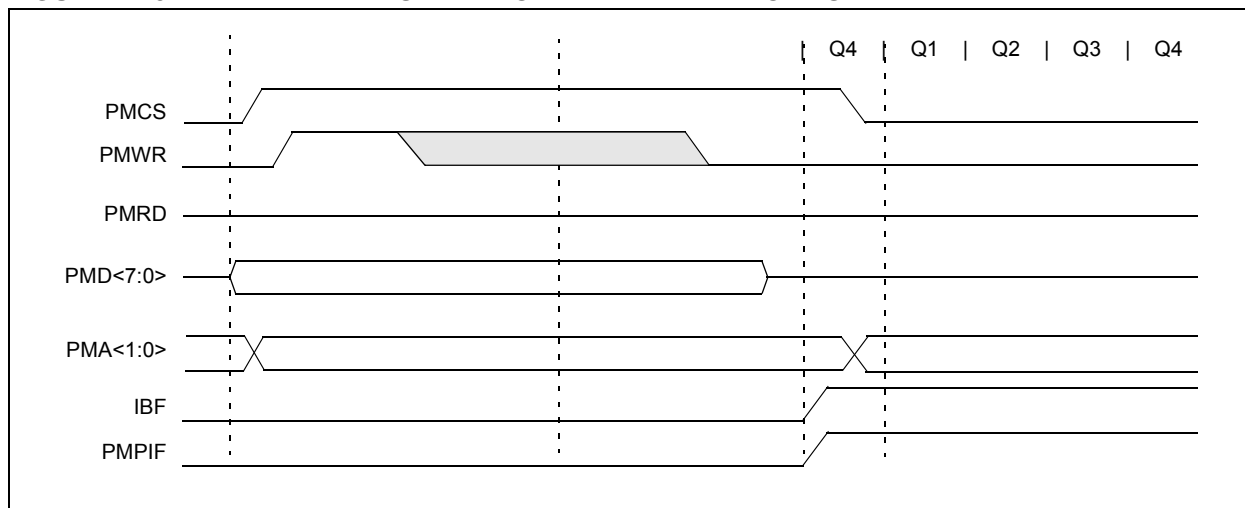
FIGURE 11-8: PARALLEL SLAVE PORT WRITE WAVEFORMS
