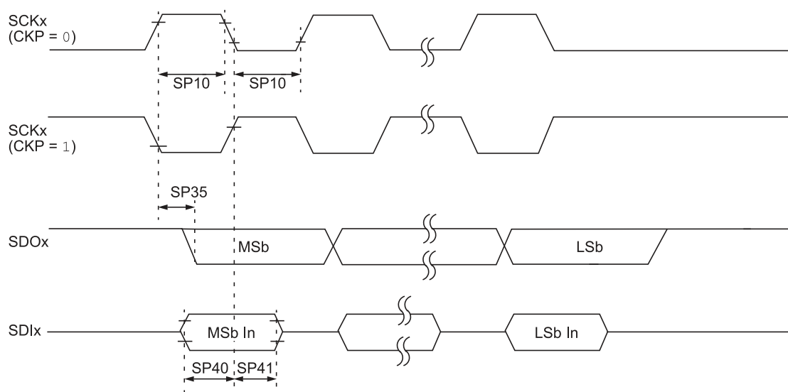
Figure 32-9. SPI Module Master Mode (CKE = 0) Timing Characteristics
