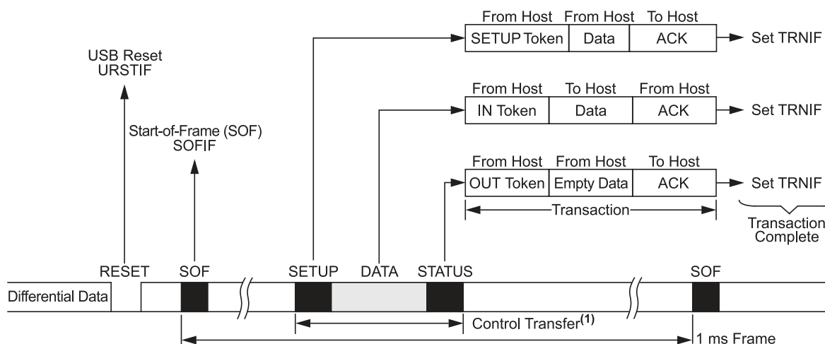
Figure 28-9. Example of a USB Transaction and Interrupt Events
