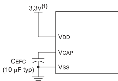
Figure 29-1. Connections for the On-Chip Regulator
