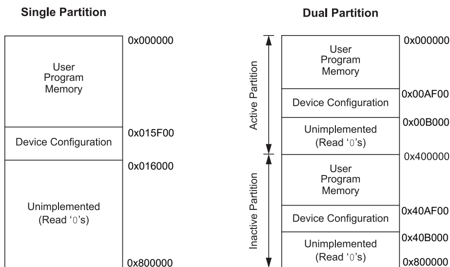
Figure 4-4. Code Memory Map for Devices with 128 Kbytes Flash (PIC24FJ128GX4XX)
