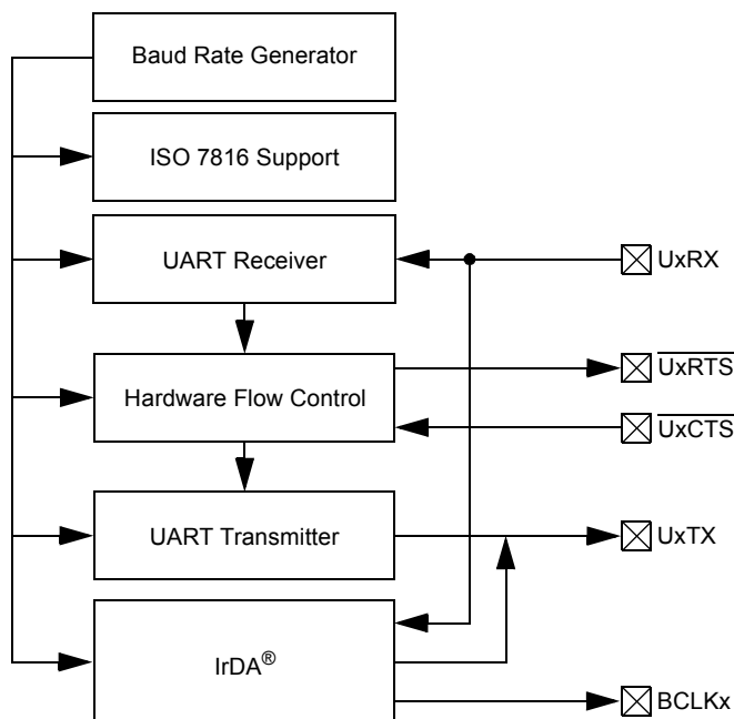
Figure 17-1. UART Simplified Block Diagram
