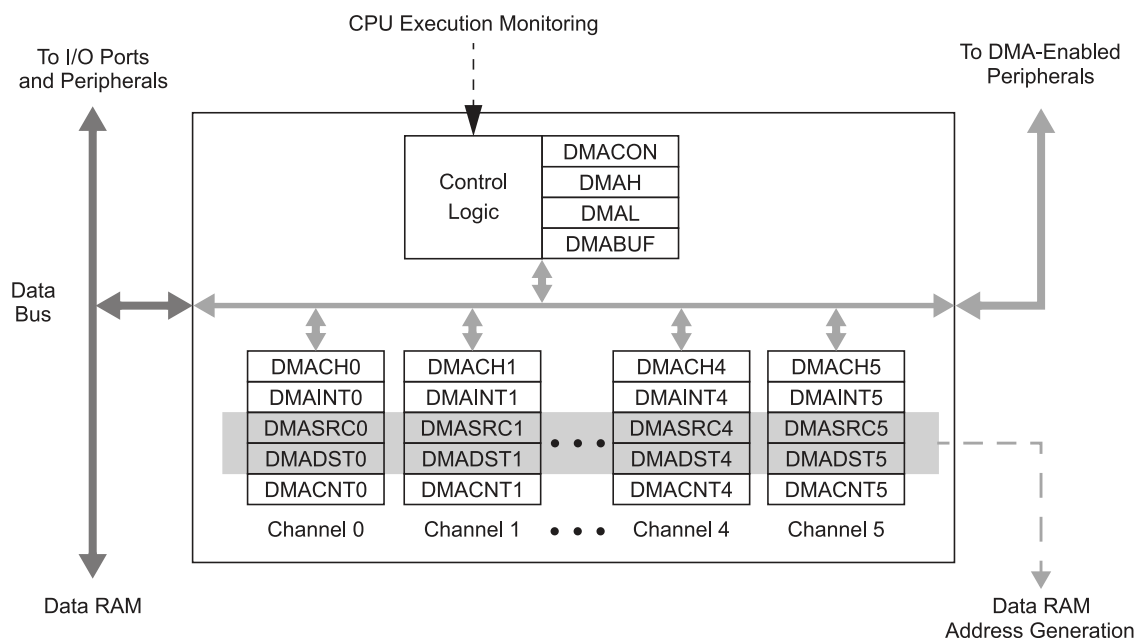
Figure 6-1. DMA Functional Block Diagram
