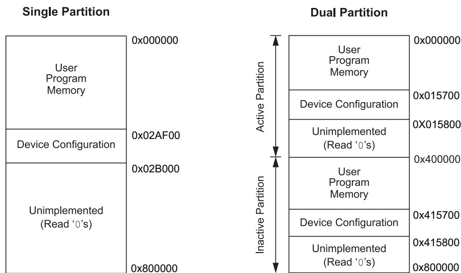
Figure 4-3. Code Memory Map for Devices with 256 Kbytes Flash (PIC24FJ256GX4XX)
