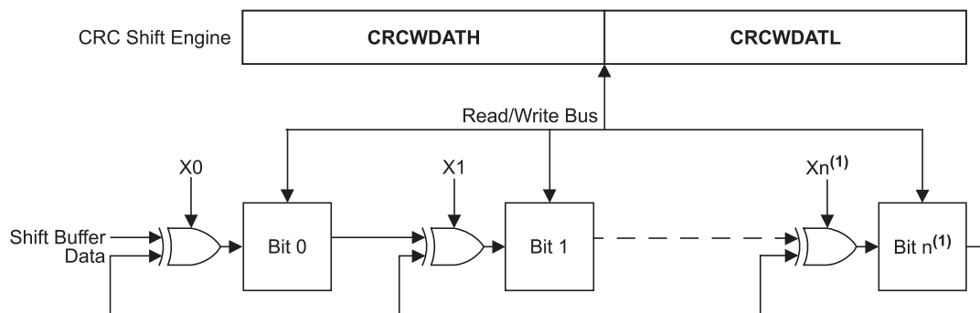
Figure 20-2. CRC Shift Engine Detail
