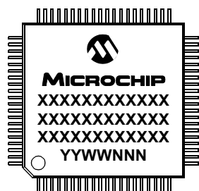
80-Lead TQFP (12x12 mm)
