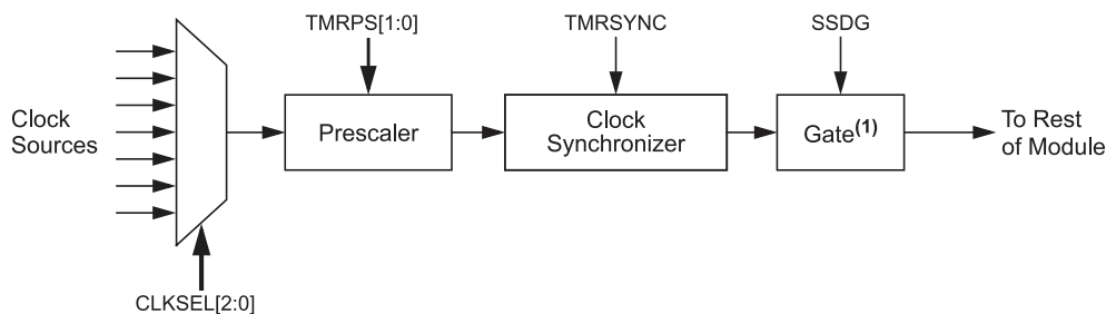
Figure 14-2. Timer Clock Generator
