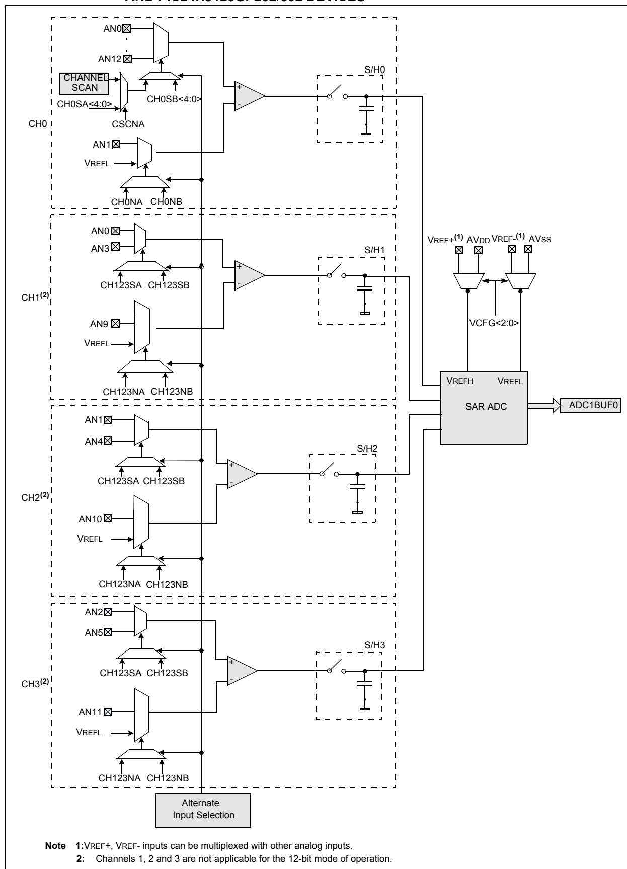
FIGURE 20-2: ADC1 MODULE BLOCK DIAGRAM FOR PIC24HJ32GP302, PIC24HJ64GP202/502 AND PIC24HJ128GP202/502 DEVICES
