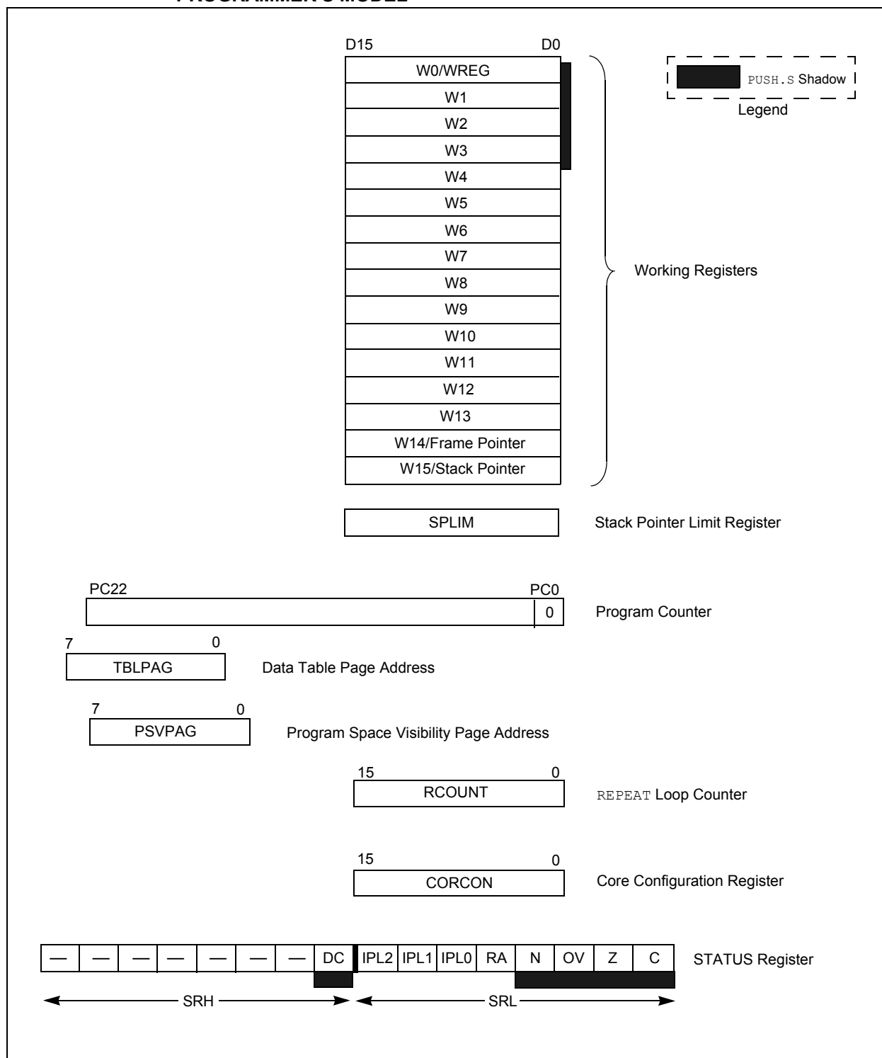
FIGURE 3-2: PIC24HJ32GP302/304, PIC24HJ64GPX02/X04 AND PIC24HJ128GPX02/X04 PROGRAMMER'S MODEL
