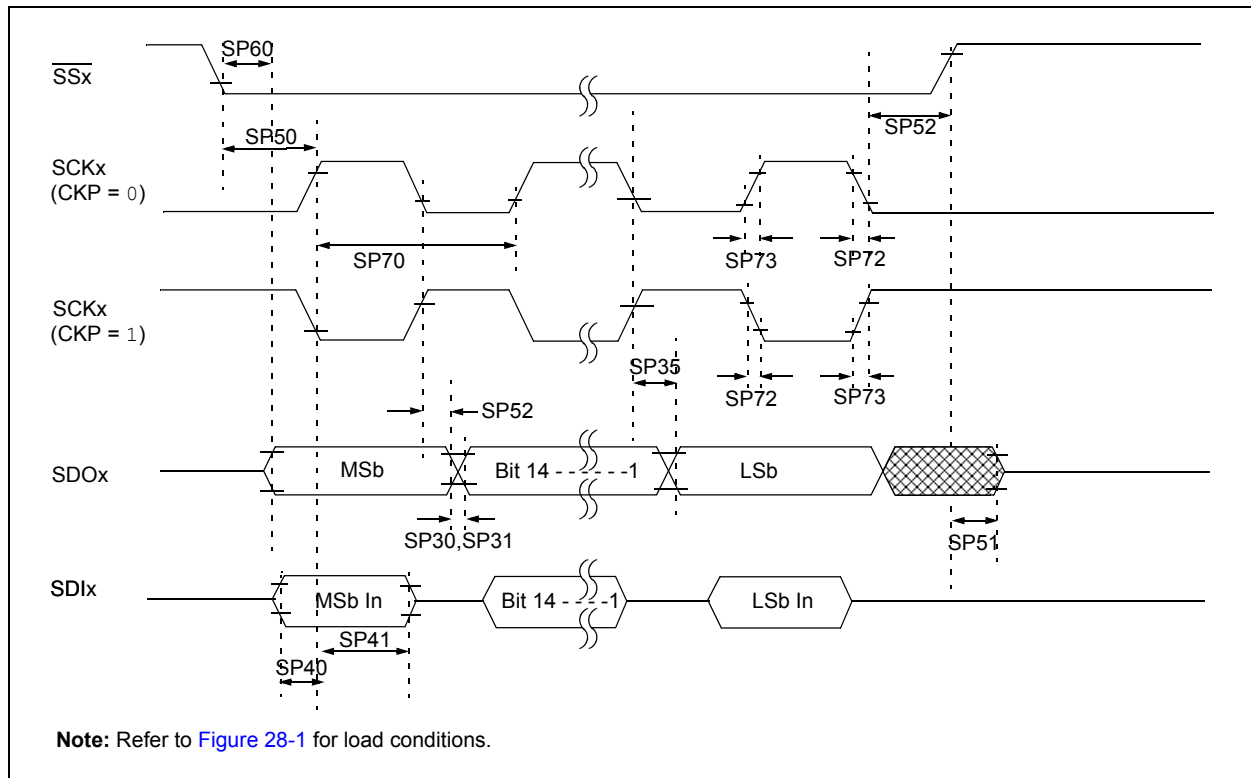
FIGURE 28-14: SPIx SLAVE MODE (FULL-DUPLEX, CKE = 1, CKP = 1, SMP = 0) TIMING CHARACTERISTICS
