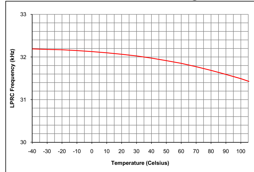
FIGURE 32-15: TYPICAL LPRC FREQUENCY @ V_{DD} = 3.3V
