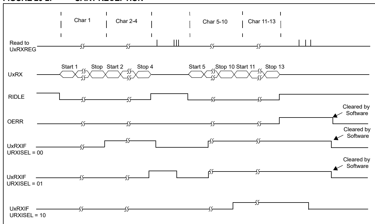
FIGURE 20-2: UART RECEPTION
