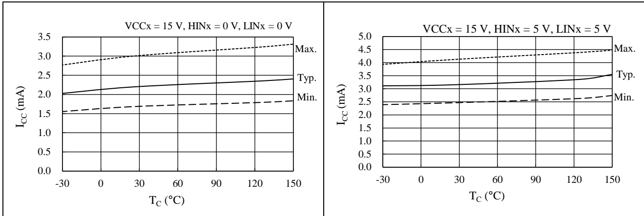
Figure 15-1. Logic Supply Current, I_{CC} vs. T_C ( I_{N_x} = 0 V)
