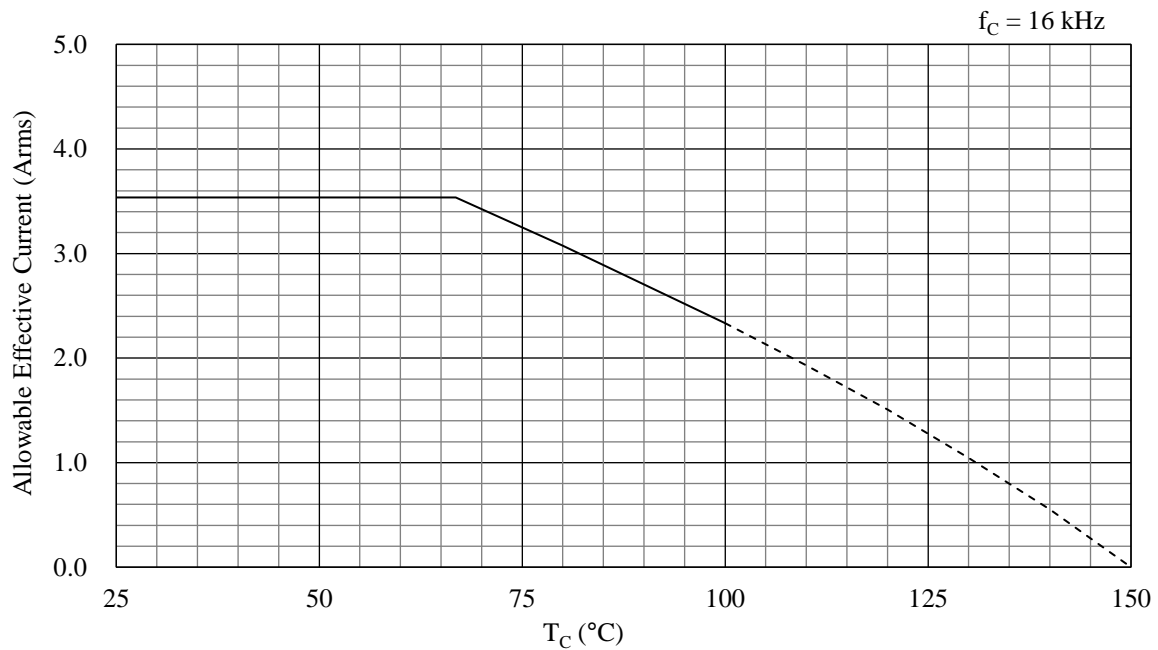
Figure 15-57. Allowable Effective Current ( f_c = 16 \text{ kHz} ): SIM6892M
