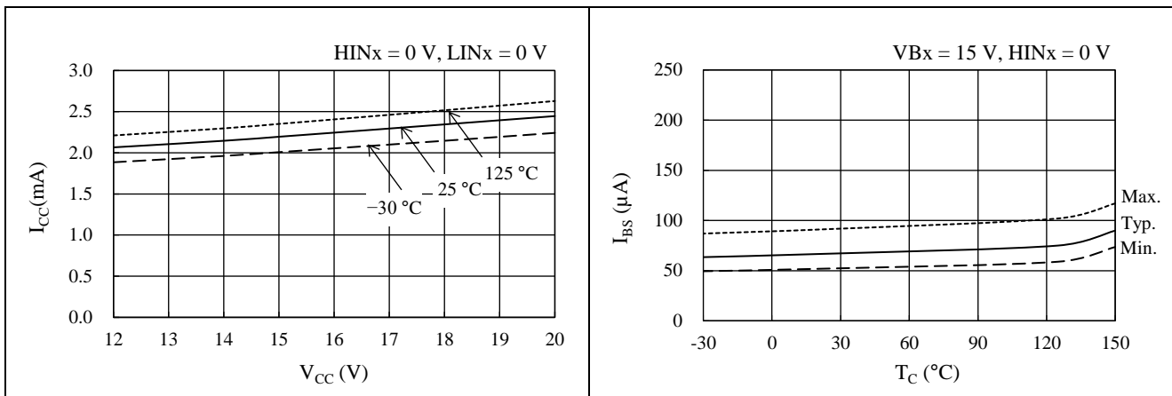
Figure 15-3. V_{CCx} Pin Voltage, V_{CC} vs. Logic Supply Current, I_{CC} curve
