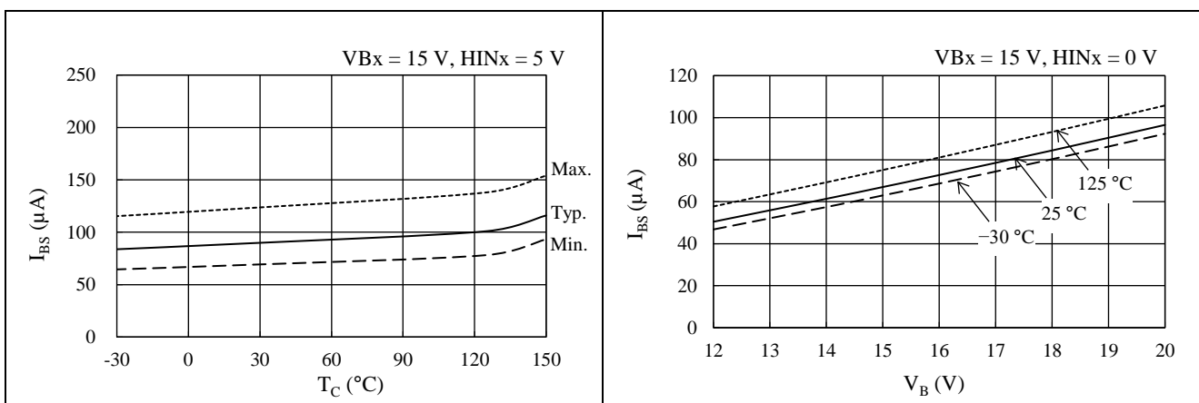
Figure 15-5. Logic Supply Current (1-phase) I_{BS} vs. T_C ( H_{INx} = 5 V)
