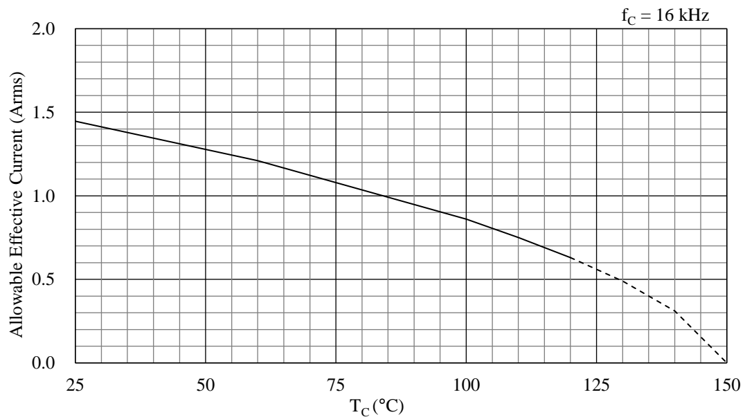
Figure 15-51. Allowable Effective Current ( f_c = 16 \text{ kHz} ): SIM6891MDN
