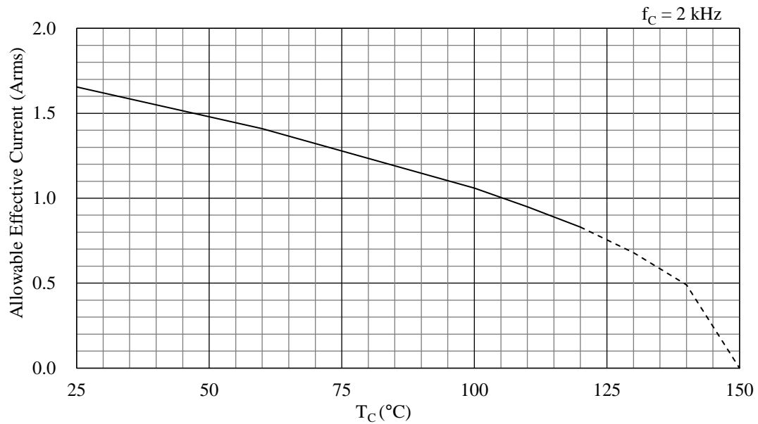
Figure 15-50. Allowable Effective Current ( f_c = 2 \text{ kHz} ): SIM6891MDN
