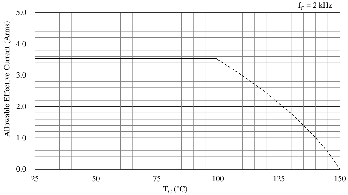
Figure 15-56. Allowable Effective Current ( f_c = 2 \text{ kHz} ): SIM6892M
