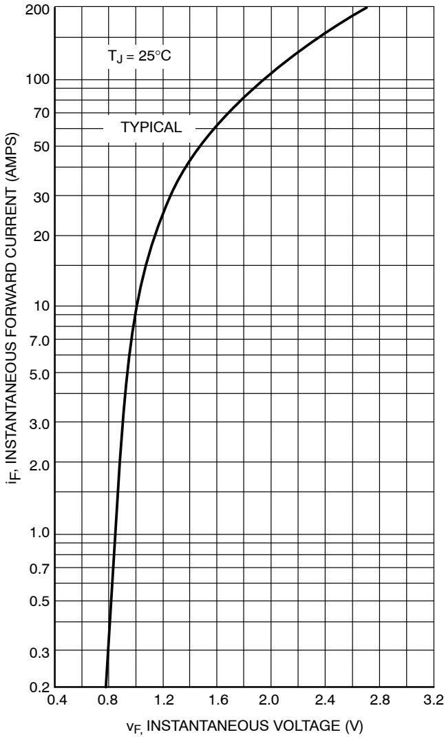
Figure 1. Forward Voltage
