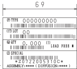
Reel label, Inner box label (unit:mm)
