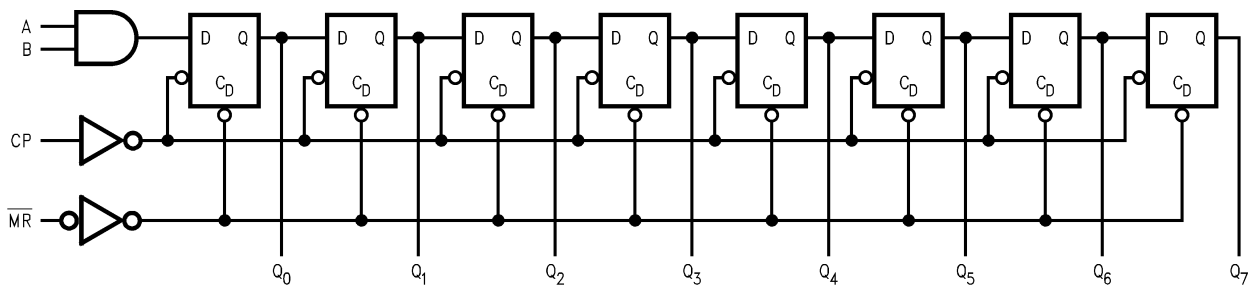
Figure 2. Logic Diagram
