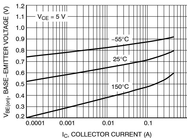
Figure 20. Base Emitter Voltage vs. Collector Current
