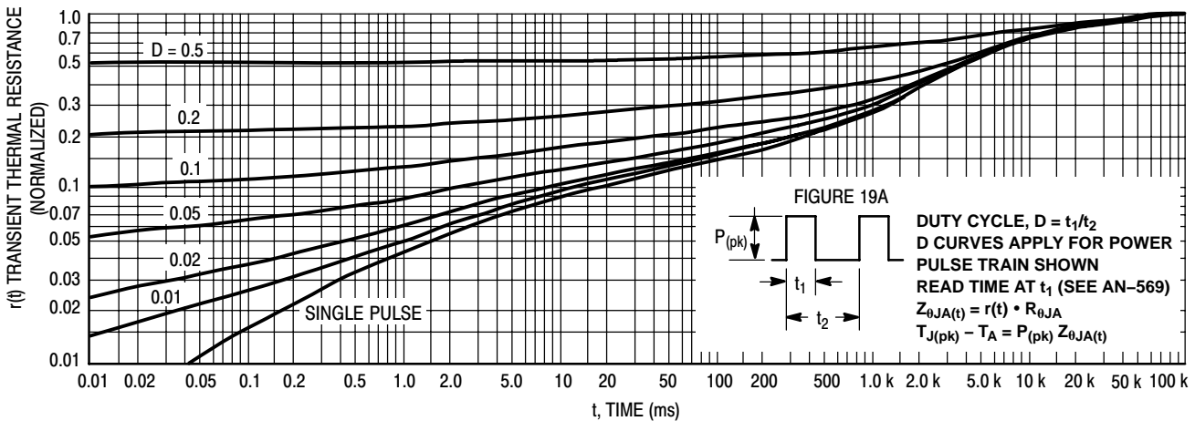
Figure 16. Thermal Response
