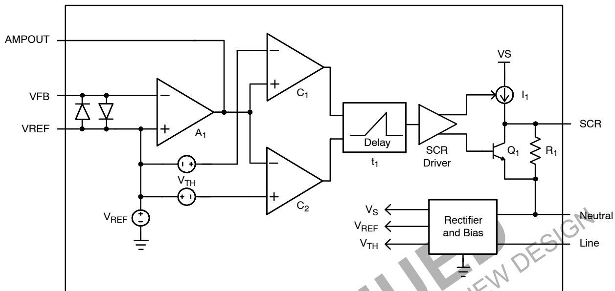
Figure 3. Block Diagram
