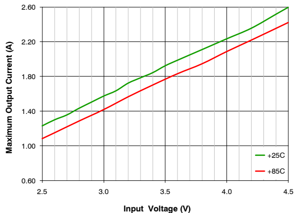
Figure 20. Typical Maximum Output Current vs. Input Voltage
