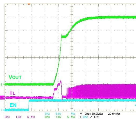
Figure 14. Startup, 50 \Omega Load
