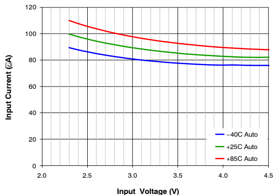
Figure 11. Quiescent Current vs. Input Voltage, Temperature
