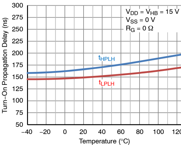
Figure 14. Turn-On Propagation Delay vs. Temp.
