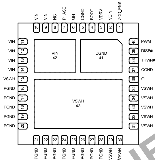
Figure 3. Top View
