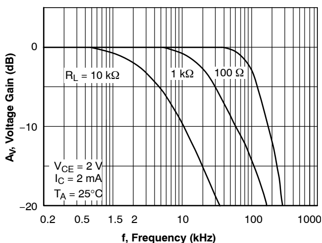
Figure 16. Frequency Response
