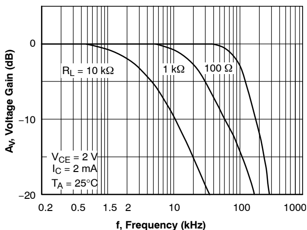
Figure 16. Frequency Response
