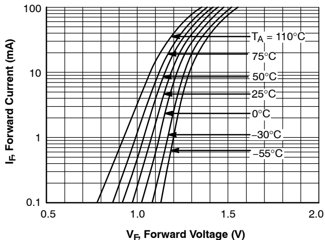
Figure 7. Forward Current vs. Forward Voltage (FOD817)
