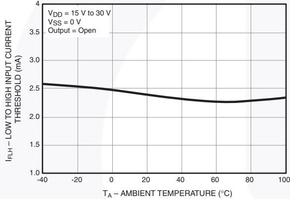
Figure 12. Low to High Input Current Threshold vs. Ambient Temperature
