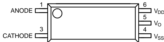
Figure 1. Pin Configuration
