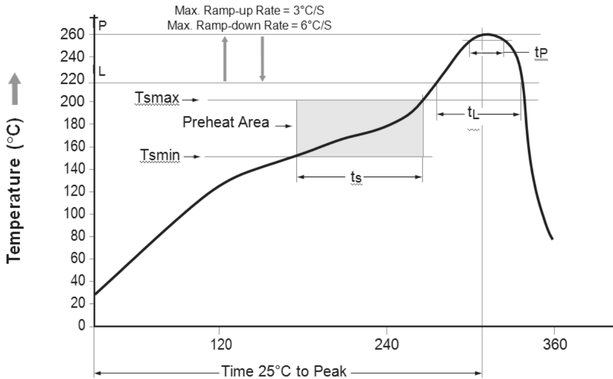
Figure 16. Reflow Profile
