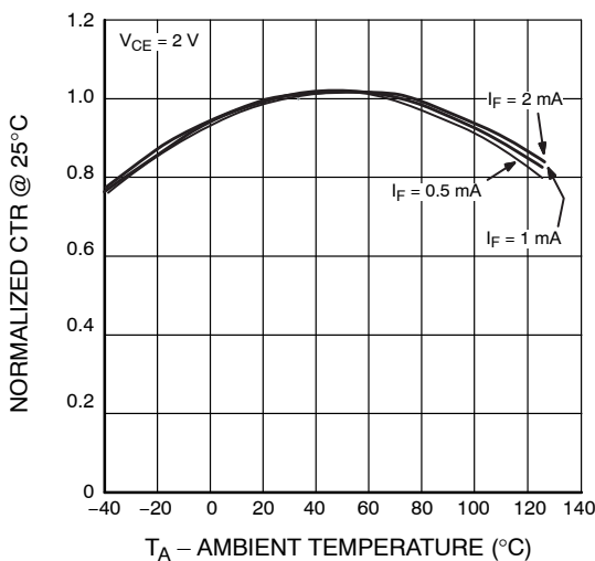
Figure 5. Normalized CTR vs. Ambient Temperature
