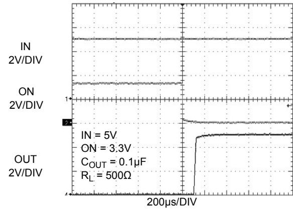
Figure 24. t_{ON} Response
