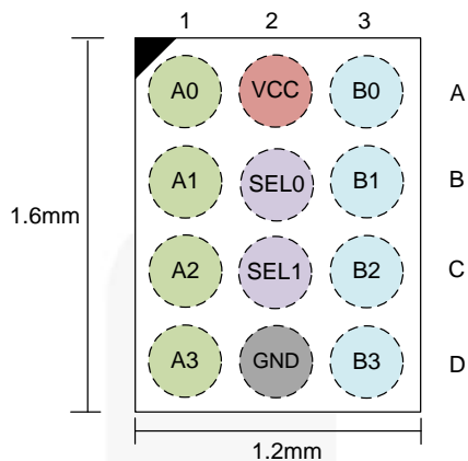
Figure 1. Pin Assignment (Top Through View)
