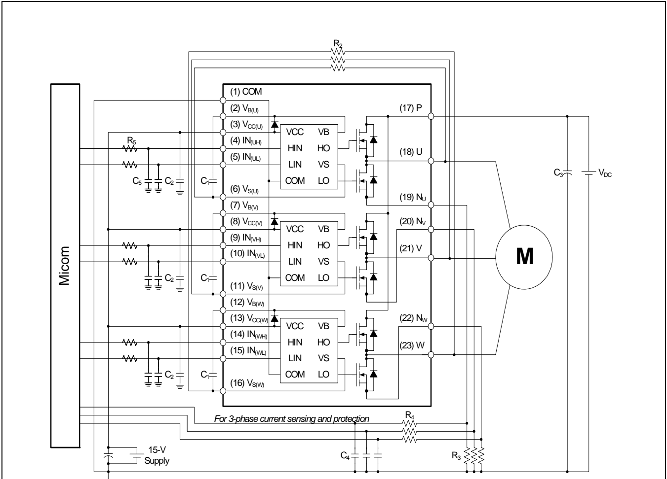
Figure 9. Example of Application Circuit
