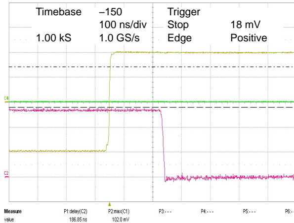
Figure 12. 100 mV Overdrive
