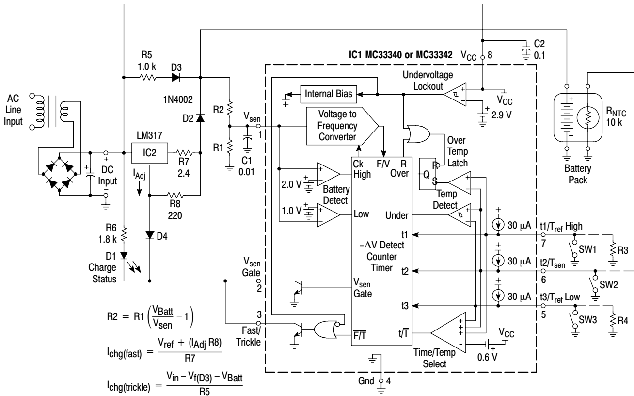
This application combines the MC33340/342 with an adjustable three terminal regulator to form an isolated secondary side battery charger. Regulator IC2 operates as a constant current source with R7 setting the fast charge level. The trickle charge level is set by R5. The R2/R1 divider should be adjusted so that the V sen input is less than 2.0 V when the batteries are fully charged. The printed circuit board shown below will accept the several TO-220 style heat-sinks for IC2 and are all manufactured by AAVID Engineering Inc.
