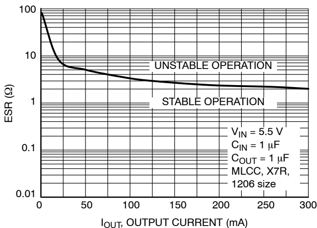
Figure 28. Output Capacitor ESR vs. Output Current
