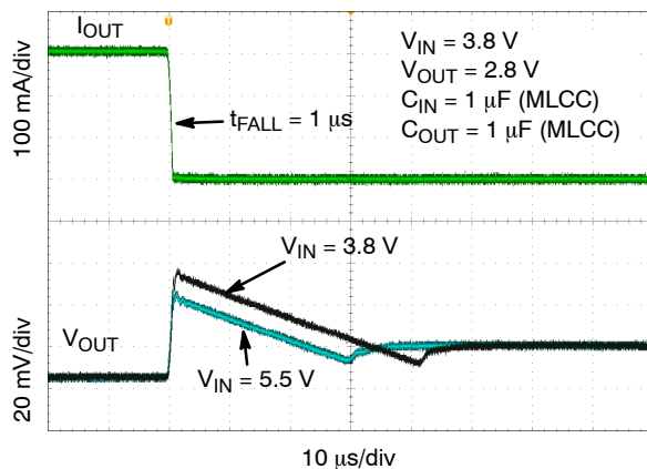
Figure 42. Load Transient Response – Falling Edge, V_{OUT} = 2.8\text{ V} , I_{OUT} = 1\text{ mA} to 300\text{ mA} , V_{IN} = 3.8\text{ V} , 5.5\text{ V}
