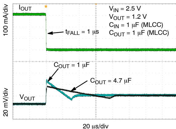
Figure 38. Load Transient Response – Falling Edge, V_{OUT} = 1.2\text{ V} , I_{OUT} = 1\text{ mA} to 300\text{ mA} , C_{OUT} = 1\text{ μF} , 4.7\text{ μF}
