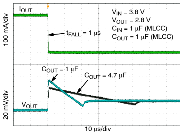
Figure 40. Load Transient Response – Falling Edge, V_{OUT} = 2.8\text{ V} , I_{OUT} = 1\text{ mA} to 300\text{ mA} , C_{OUT} = 1\text{ μF} , 4.7\text{ μF}
