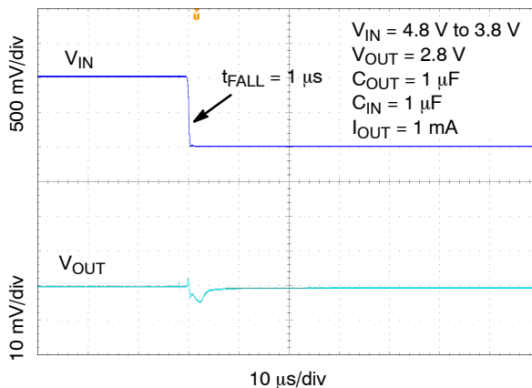
Figure 34. Line Transient Response – Falling Edge, V_{OUT} = 2.8\text{ V} , I_{OUT} = 1\text{ mA}
