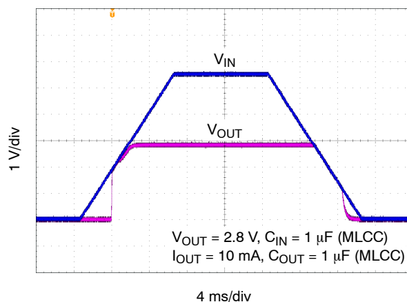
Figure 42. Turn-on/off – Slow Rising V_{IN}
