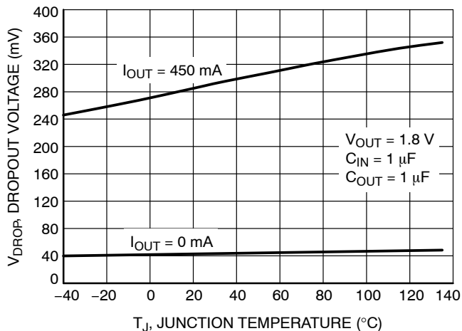
Figure 21. Dropout Voltage vs. Temperature – V_{OUT} = 1.8\text{ V}
