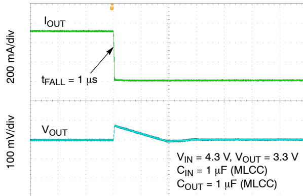
Figure 46. Load Transient Response – 450 mA to 1 mA – V_{OUT} = 3.3\text{ V}
