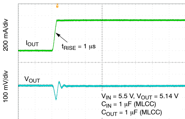
Figure 47. Load Transient Response – 1 mA to 450 mA – V_{OUT} = 5.14\text{ V}
