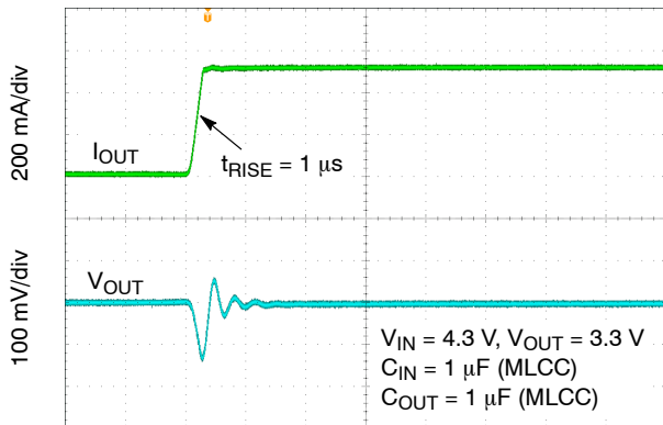
Figure 45. Load Transient Response – 1 mA to 450 mA – V_{OUT} = 3.3\text{ V}
