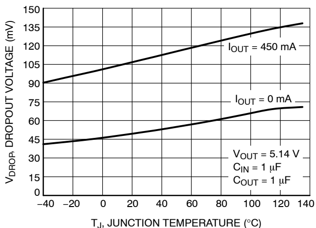
Figure 23. Dropout Voltage vs. Temperature – V_{OUT} = 5.14\text{ V}
