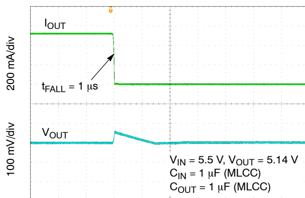
Figure 48. Load Transient Response – 450 mA to 1 mA – V_{OUT} = 5.14\text{ V}
