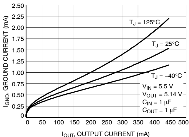
Figure 17. Ground Current vs. Load Current – V_{OUT} = 5.14\text{ V}
