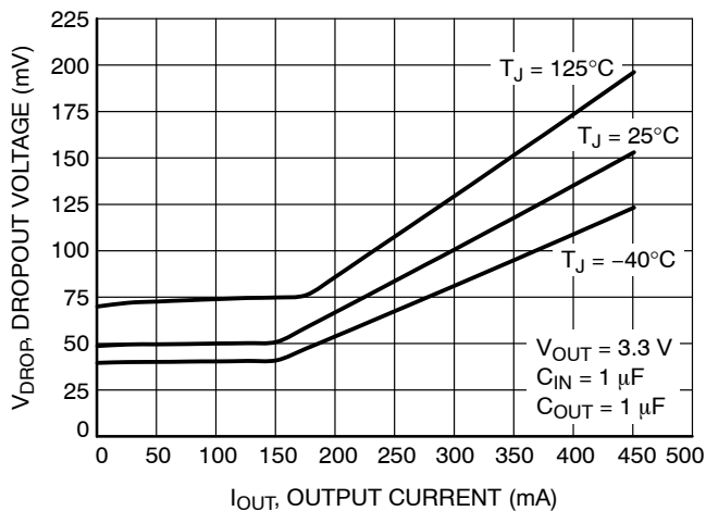
Figure 19. Dropout Voltage vs. Load Current – V_{OUT} = 3.3\text{ V}
