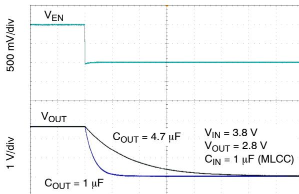
Figure 50. Enable Turn-off
