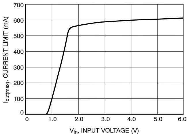
Figure 23. Current Limit vs. Input Voltage
