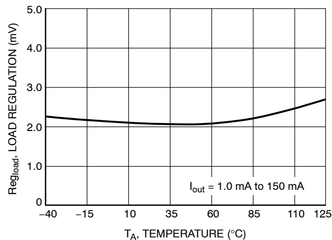
Figure 25. Load Regulation vs. Temperature
