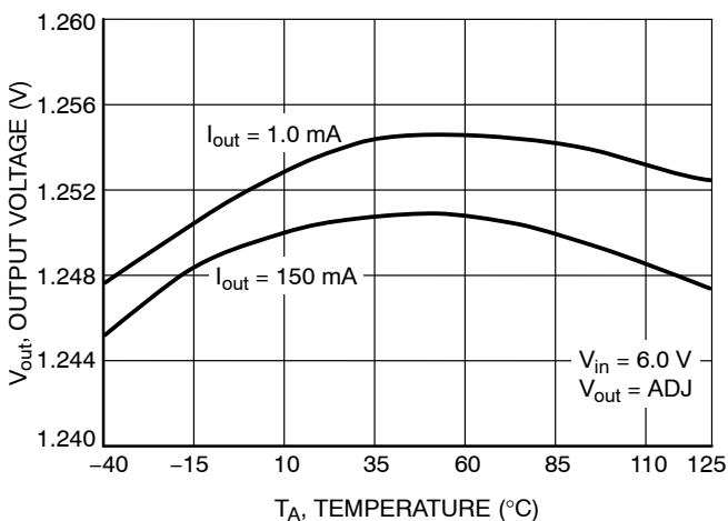
Figure 6. Output Voltage vs. Temperature ( V_{in} = 6.0 V )
