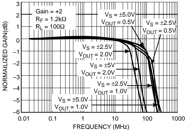
Figure 5. Frequency Response: Gain (dB) vs. Frequency A v = +2.0
