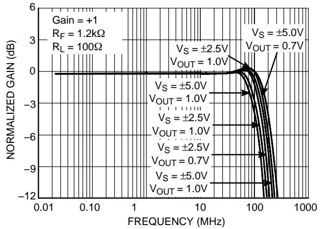
Figure 6. Frequency Response: Gain (dB) vs. Frequency A v = +1.0
