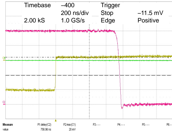
Figure 16. 10 mV Overdrive
