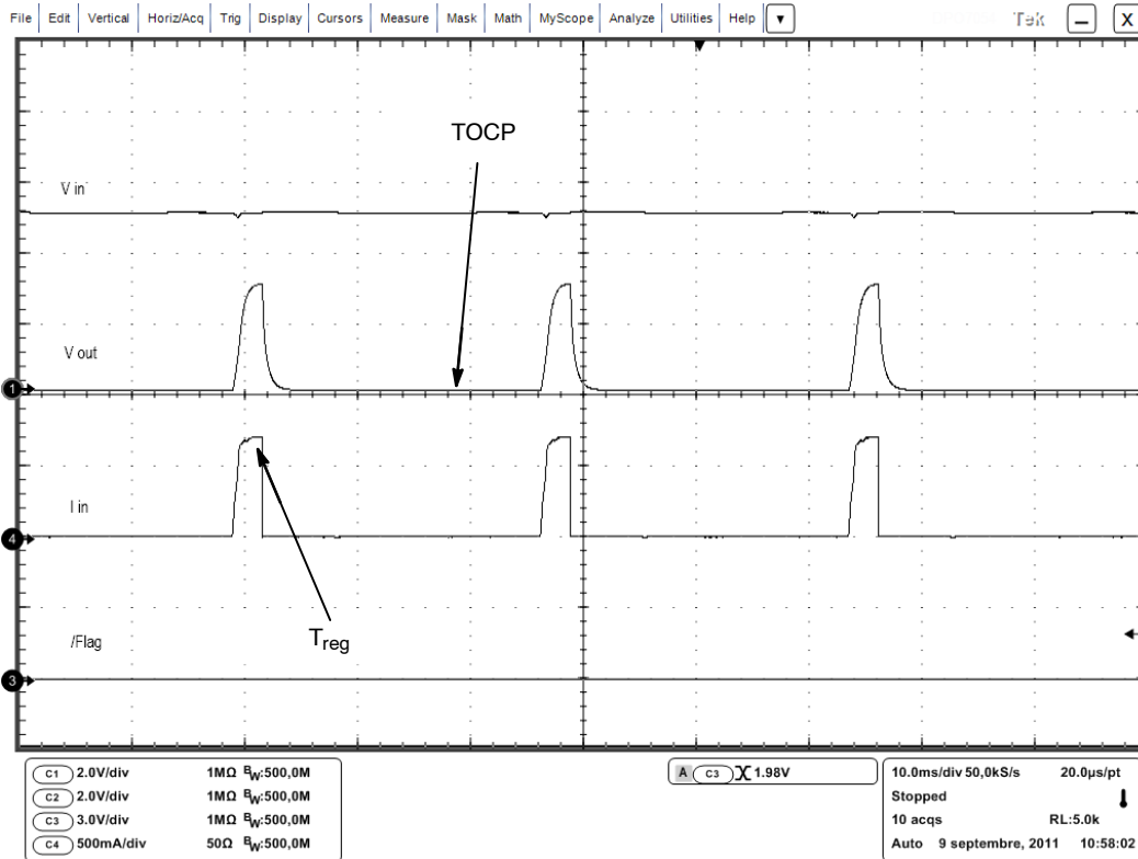
Figure 11. Timer Regulation Sequence During 2 Ohm Overload
