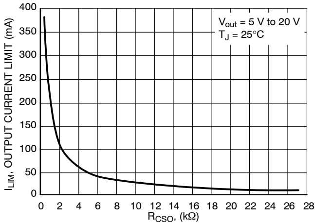
Figure 9. Output Current Limit vs. R_{CSO}
