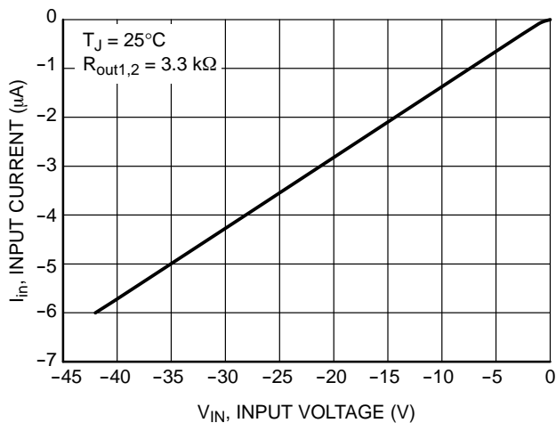
Figure 7. Input Current vs. Input Voltage (Reverse Input Voltage)
