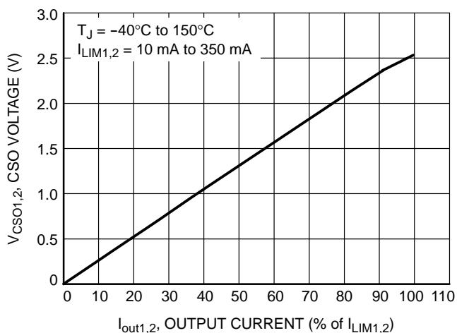
Figure 9. CSO Voltage vs. Output Current (% of I LIM )
