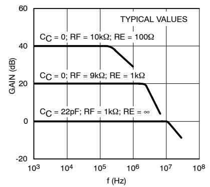
Figure 4. Closed-Loop Frequency Response
