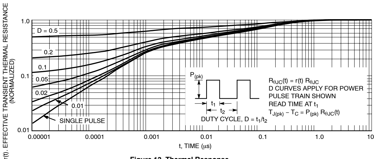
Figure 13. Thermal Response
