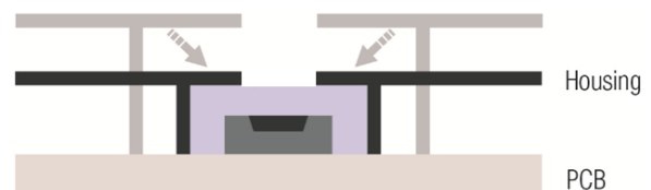
Figure 3: A small dead volume allows for rapid adaption to changes in the environment.
