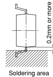
Soldering area
