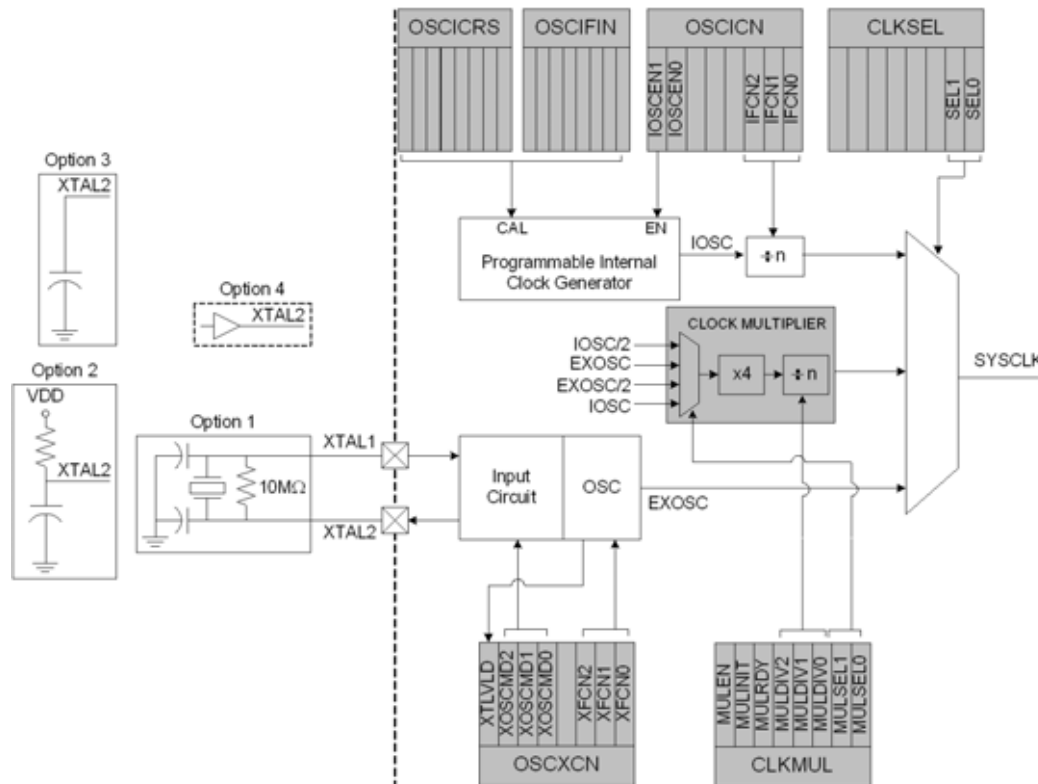
Figure 19.1. Oscillator Options
