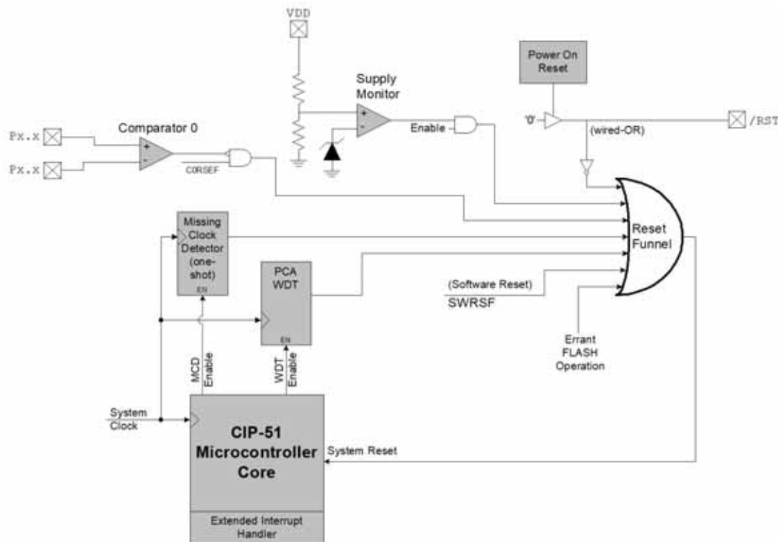
Figure 17.1. Reset Sources
