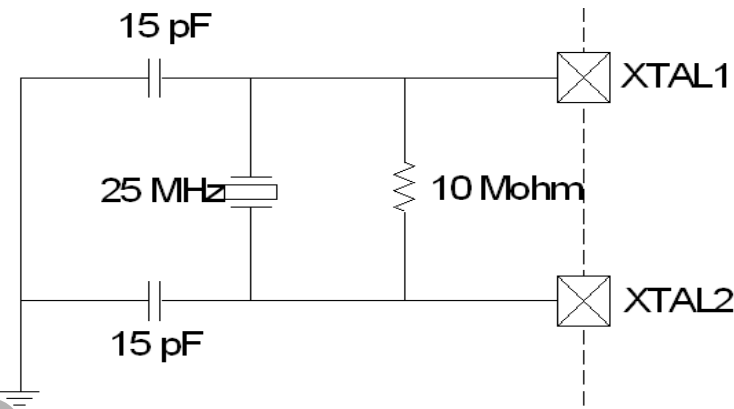
Figure 23.2. 25 MHz External Crystal Example
