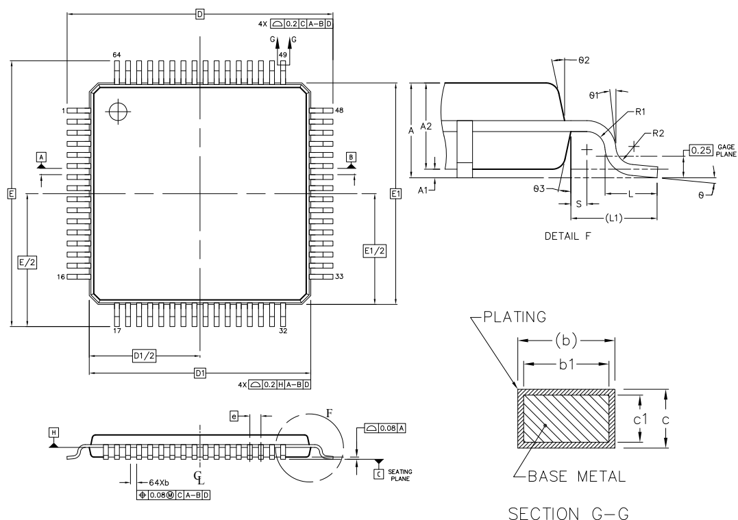
Figure 9.1. TQFP64
