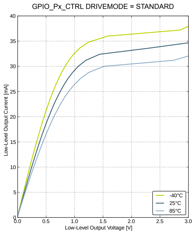
Figure 4.12. Typical Low-Level Output Current, 3 V Supply Voltage
