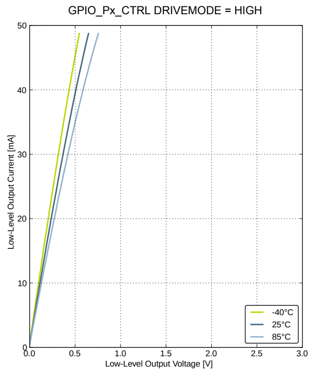
Figure 4.12. Typical Low-Level Output Current, 3 V Supply Voltage
