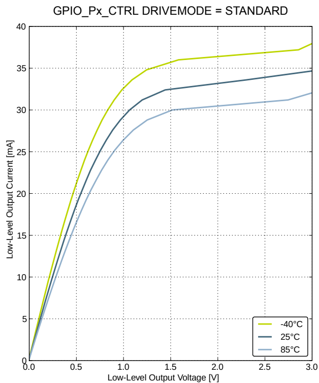
Figure 4.12. Typical Low-Level Output Current, 3 V Supply Voltage
