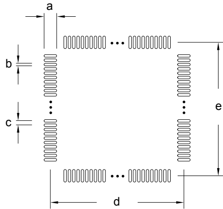
Figure 8.4. LQFP100 PCB Stencil Design
