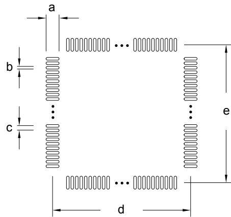
Figure 9.4. TQFP64 PCB Stencil Design
